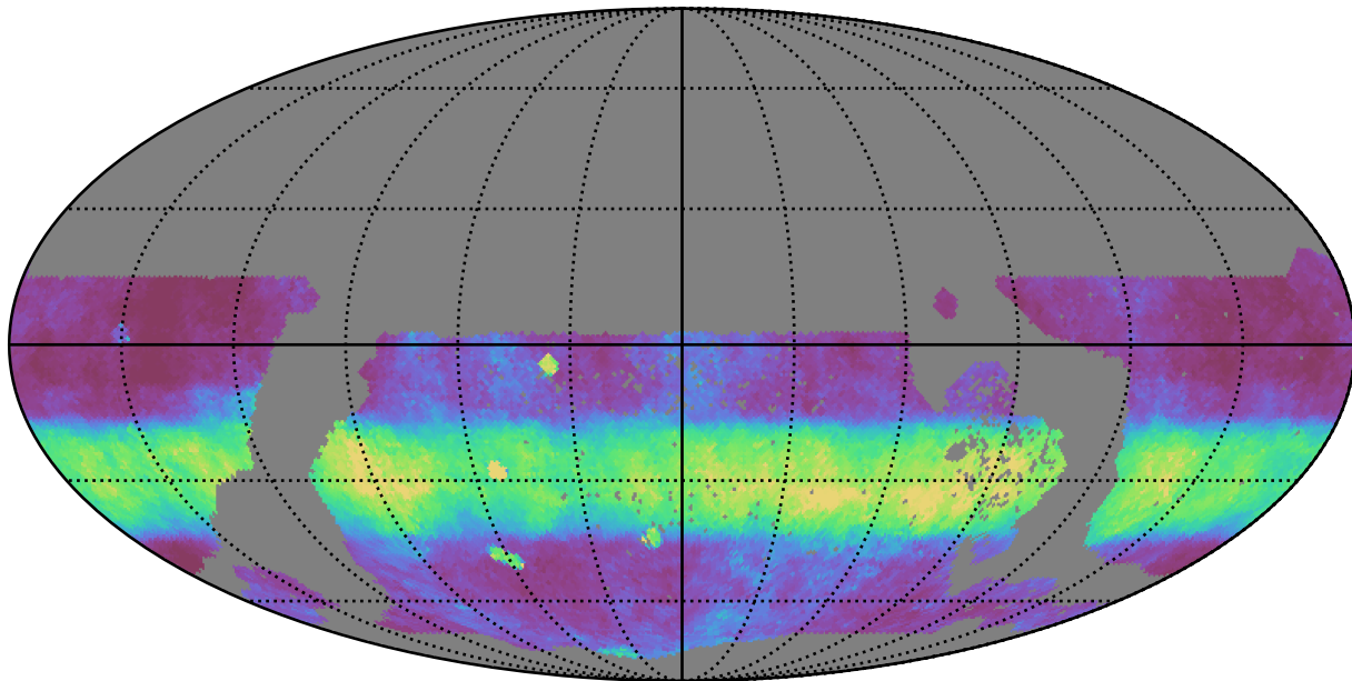
weather_cloudso0v3.4_10yrs WFD i band: Median normairmass
