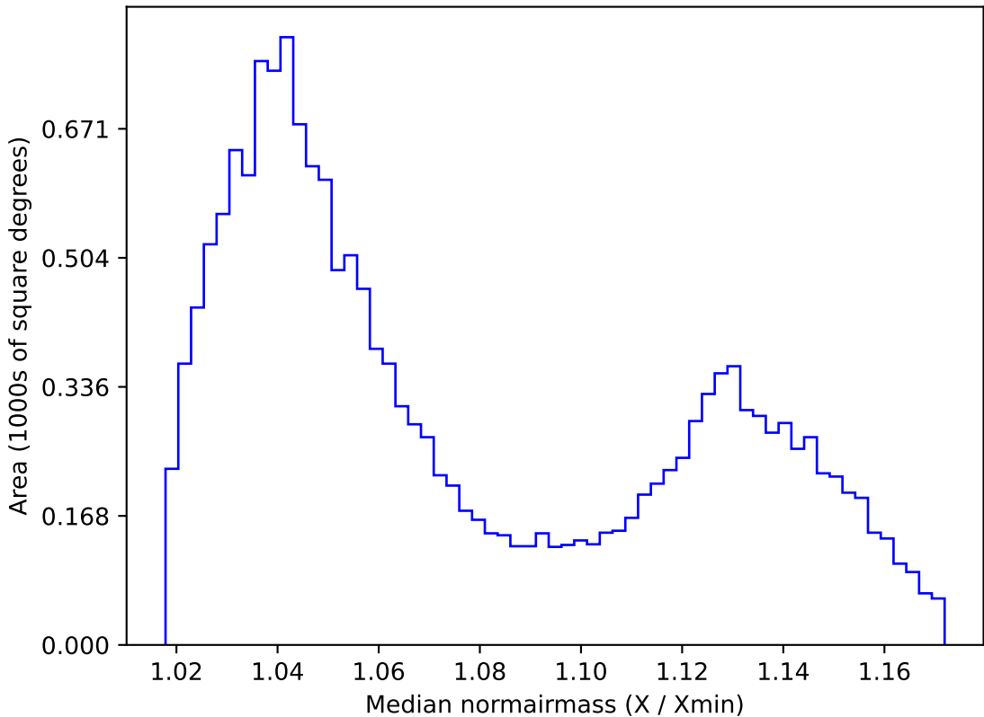
weather_cloudso0v3.4_10yrs WFD i band: Median normairmass
