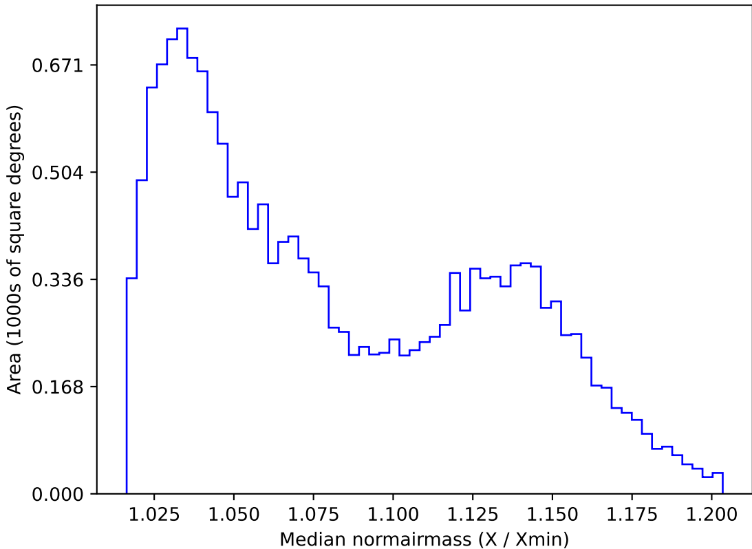
weather_cloudso0v3.4_10yrs WFD g band: Median normairmass
