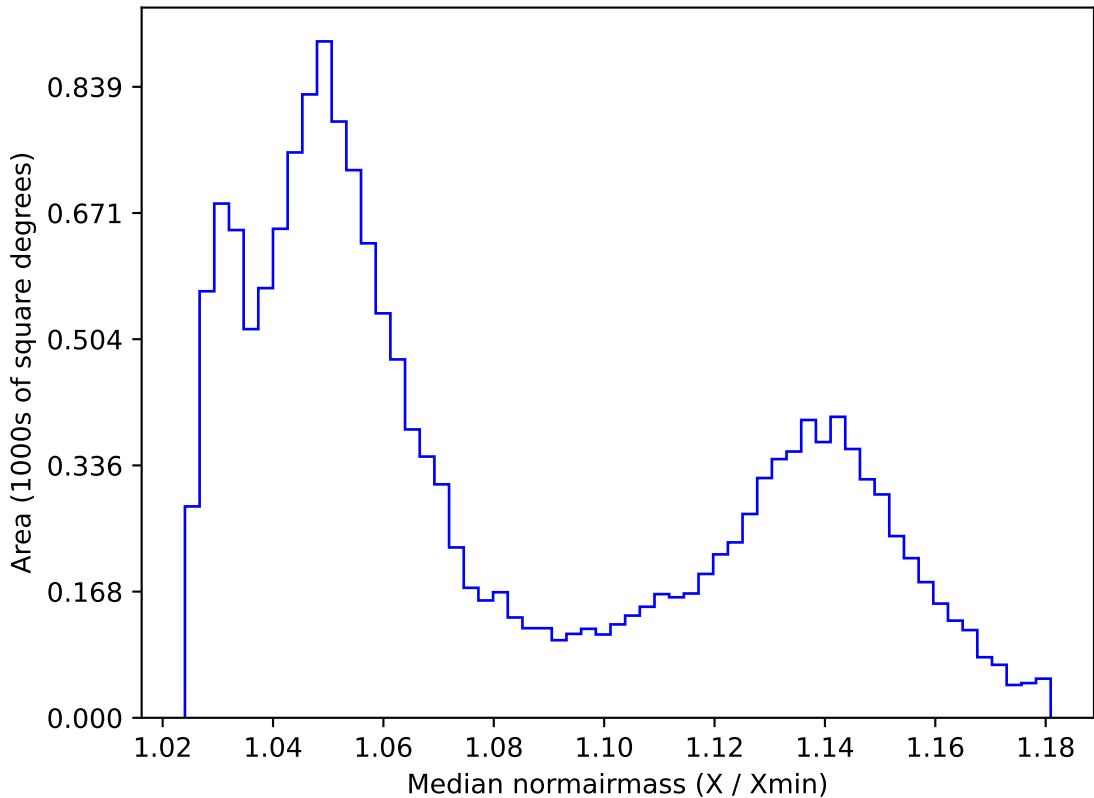
weather_cloudso0v3.4_10yrs WFD all bands: Median normairmass
