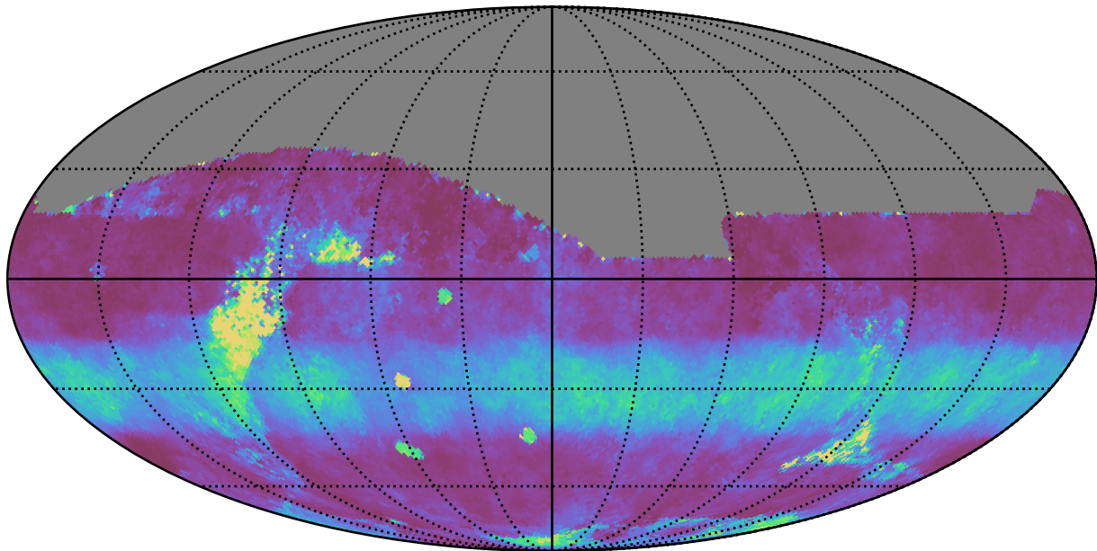
weather_cloudso0v3.4_10yrs All sky z band: Median normairmass
