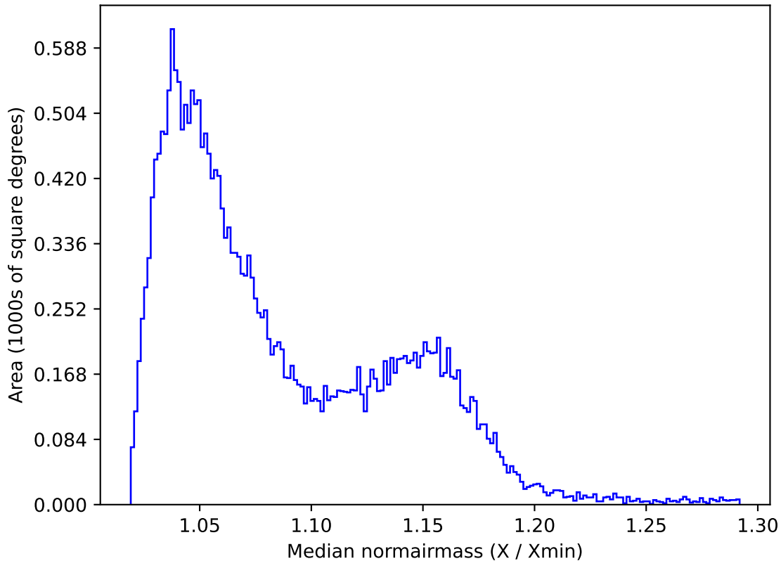
weather_cloudso0v3.4_10yrs All sky z band: Median normairmass
