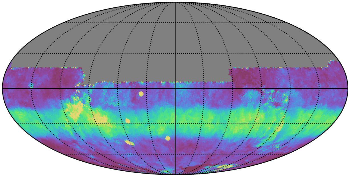
weather_cloudso0v3.4_10yrs All sky y band: Median normairmass
