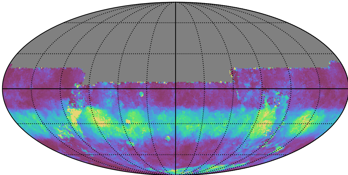
weather_cloudso0v3.4_10yrs All sky u band: Median normairmass
