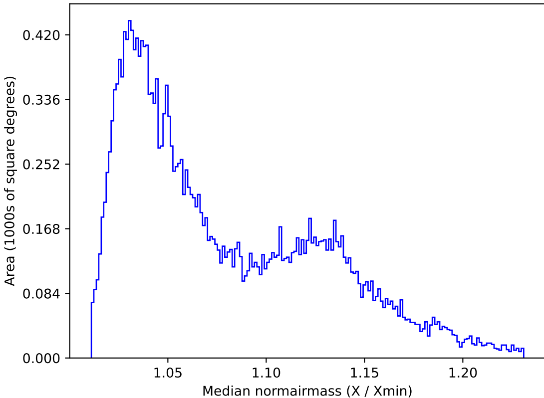
weather_cloudso0v3.4_10yrs All sky u band: Median normairmass
