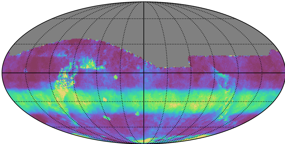
weather_cloudso0v3.4_10yrs All sky i band: Median normairmass
