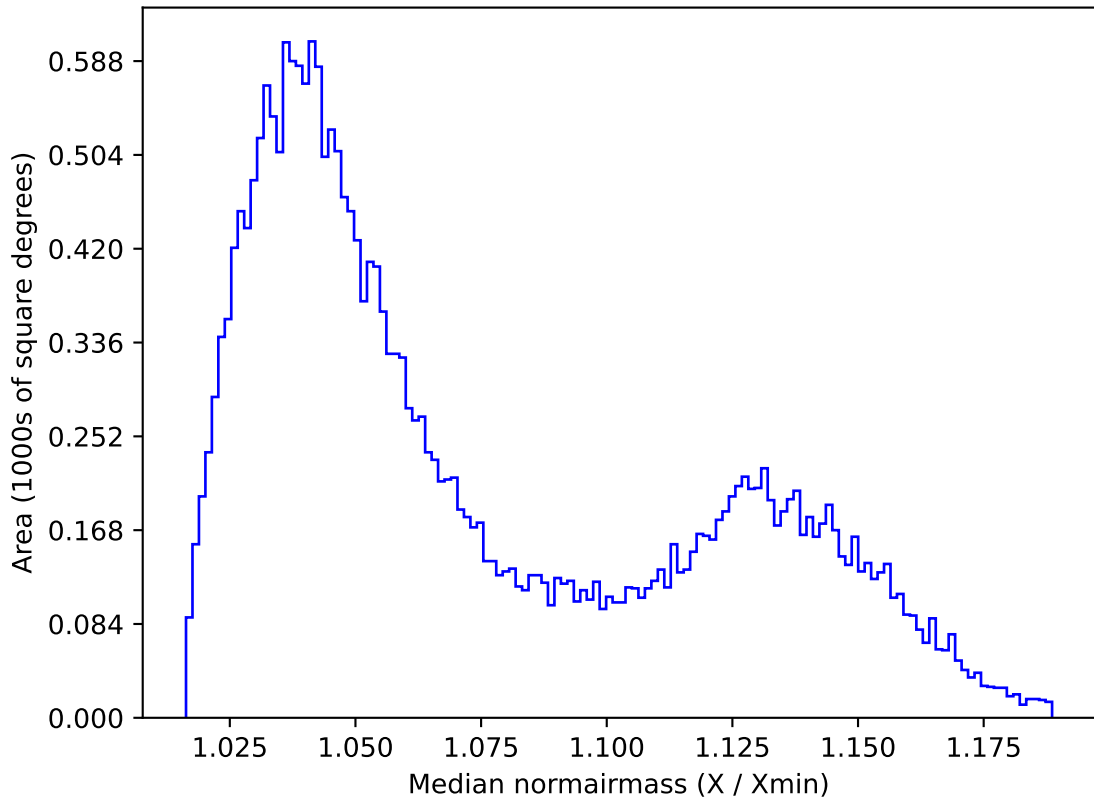
weather_cloudso0v3.4_10yrs All sky i band: Median normairmass
