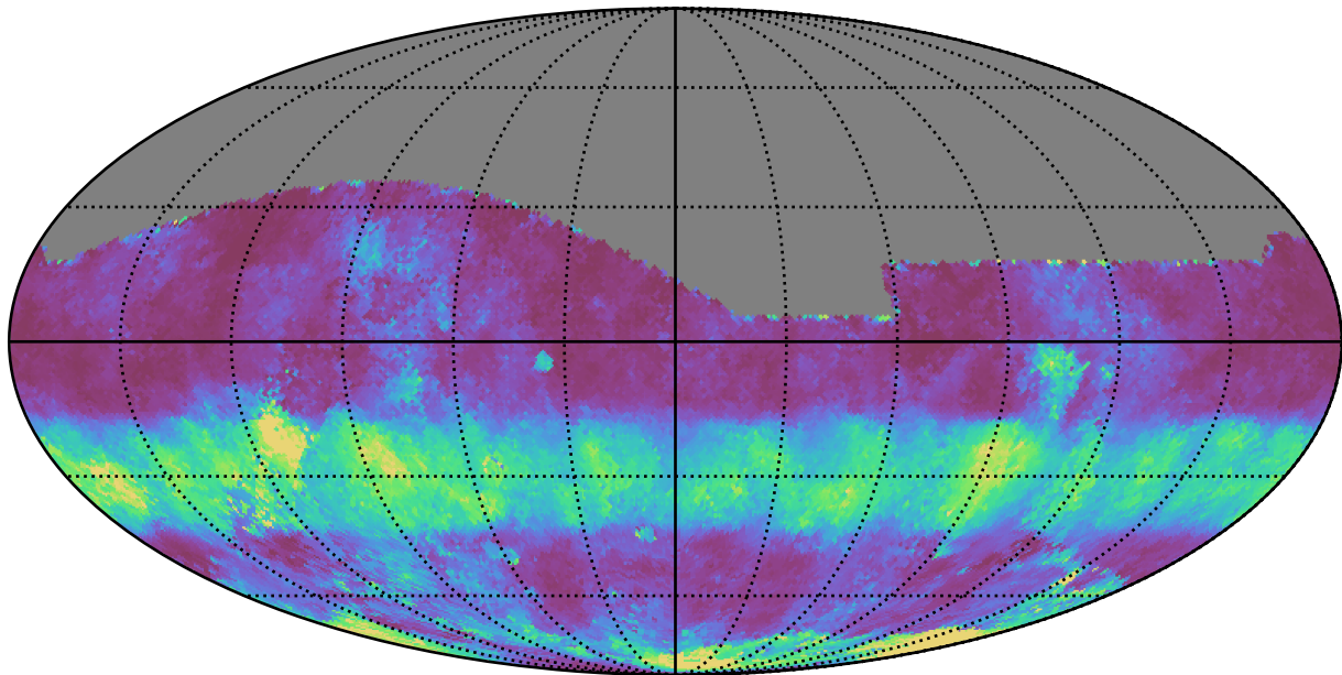
weather_cloudso0v3.4_10yrs All sky g band: Median normairmass
