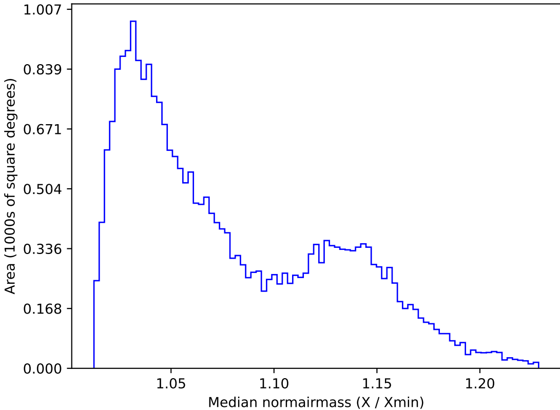
weather_cloudso0v3.4_10yrs All sky g band: Median normairmass
