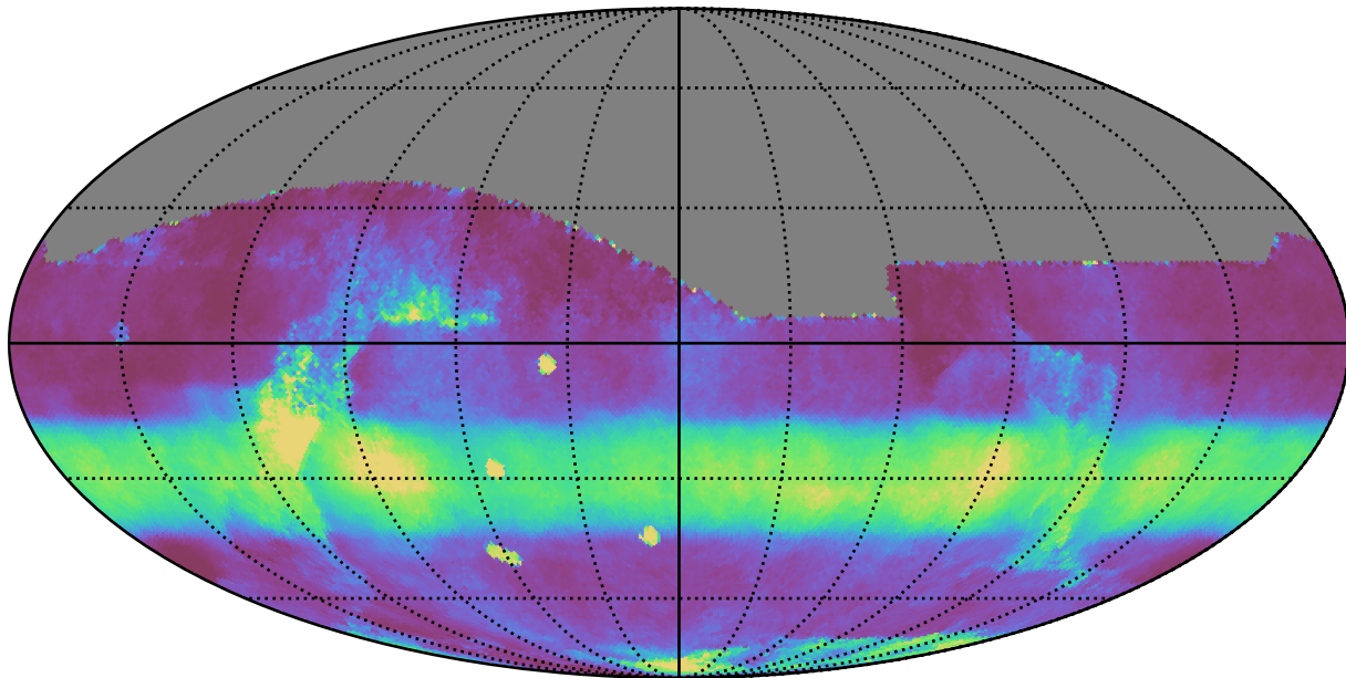
weather_cloudso0v3.4_10yrs All sky all bands: Median normairmass
