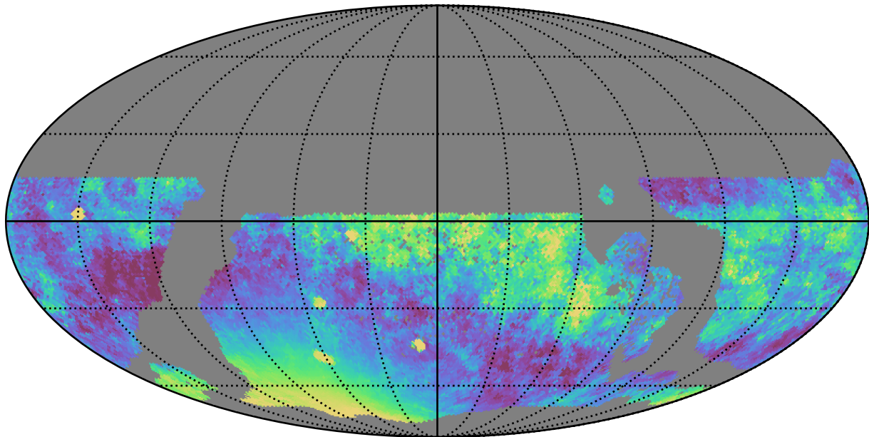
weather_cloudso0v3.4_10yrs WFD z band: Median moonDistance
