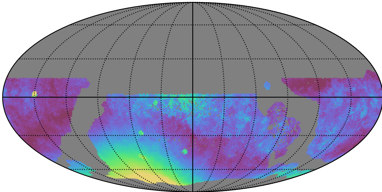
weather_cloudso0v3.4_10yrs WFD y band: Median moonDistance
