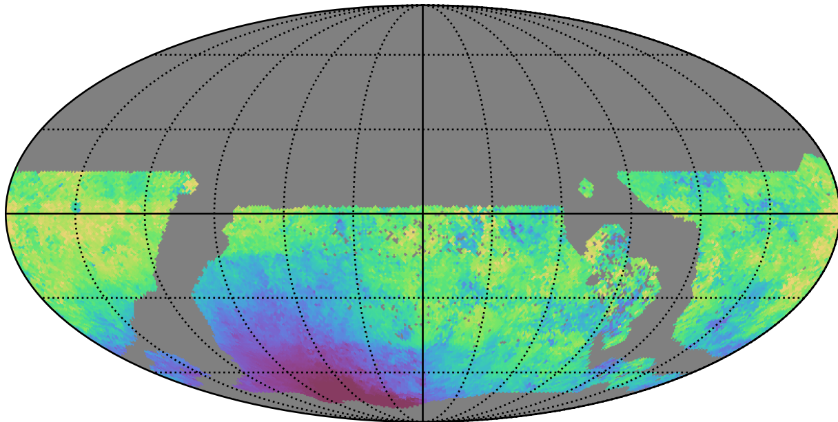
weather_cloudso0v3.4_10yrs WFD u band: Median moonDistance
