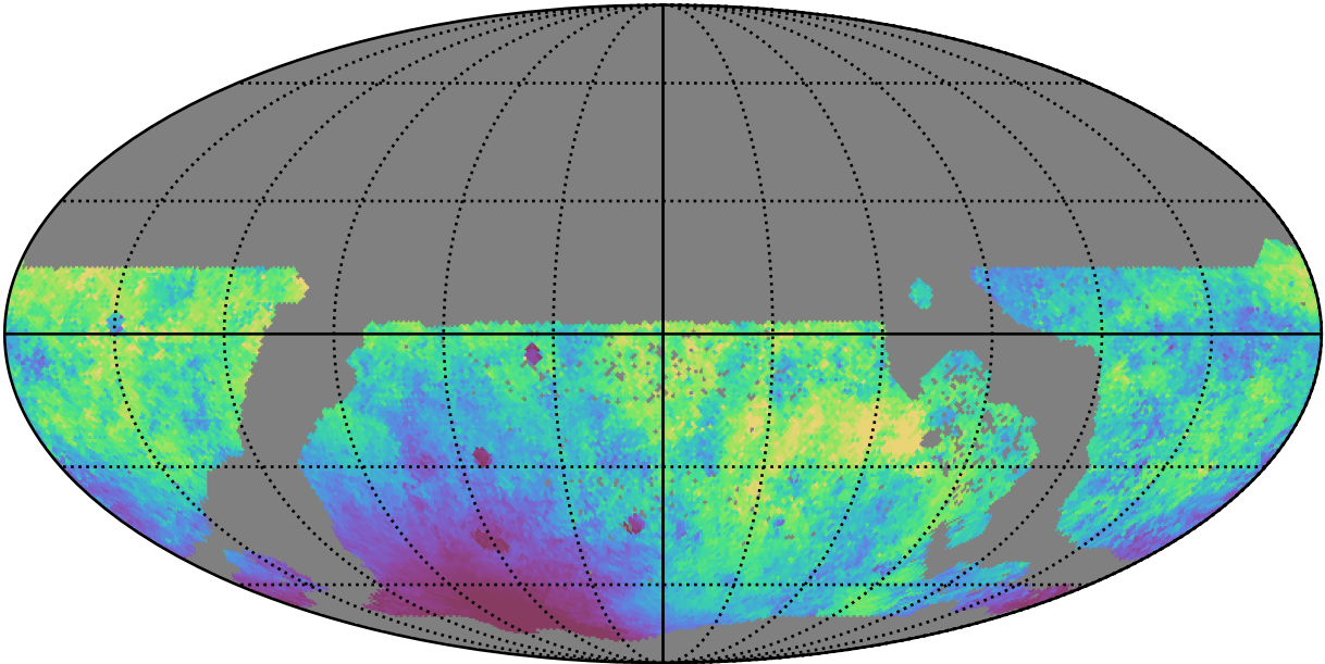
weather_cloudso0v3.4_10yrs WFD r band: Median moonDistance
