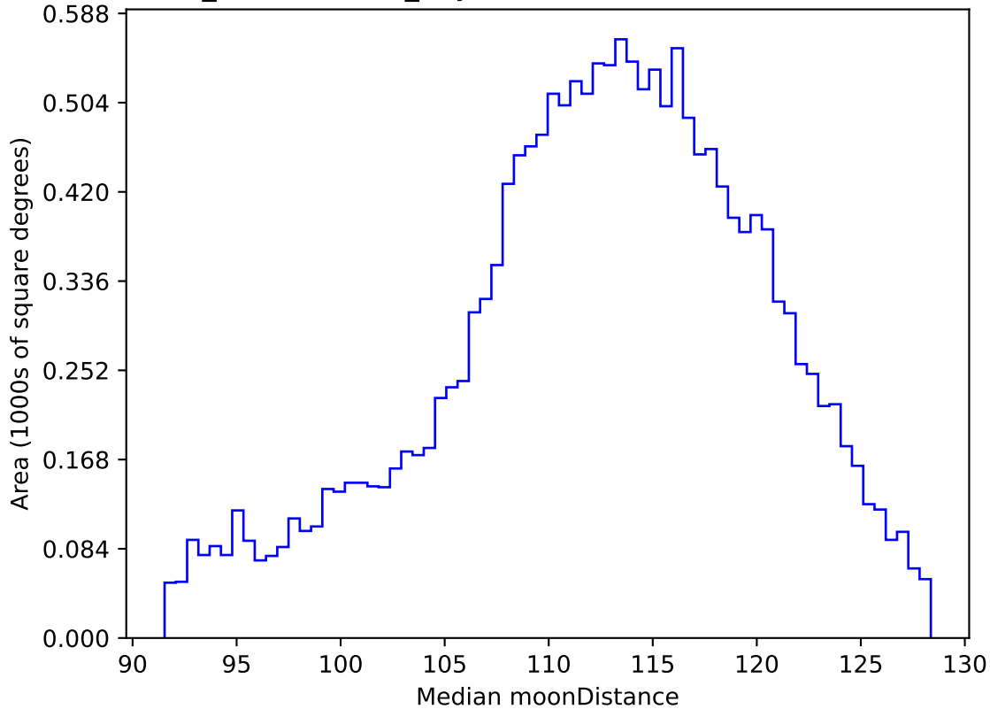
weather_cloudso0v3.4_10yrs WFD r band: Median moonDistance
