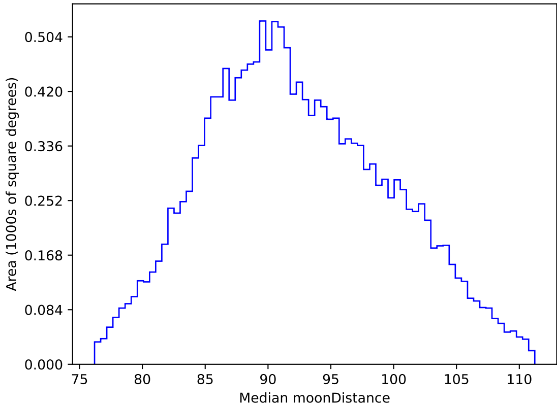
weather_cloudso0v3.4_10yrs WFD i band: Median moonDistance
