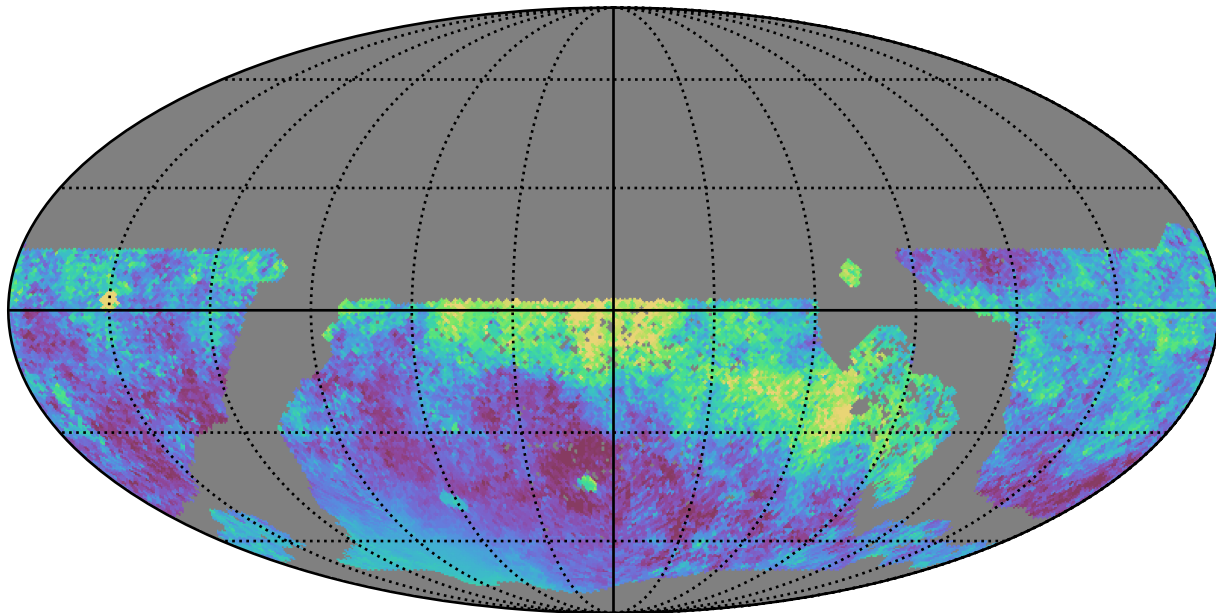
weather_cloudso0v3.4_10yrs WFD all bands: Median moonDistance
