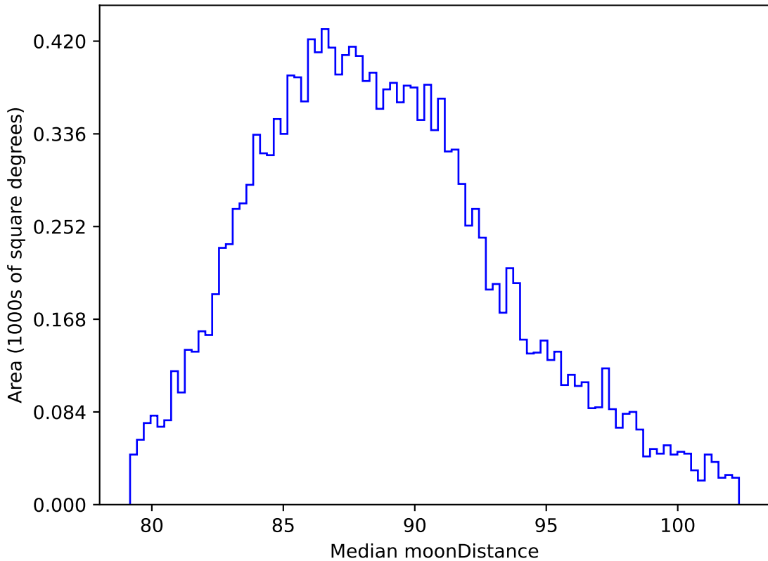
weather_cloudso0v3.4_10yrs WFD all bands: Median moonDistance
