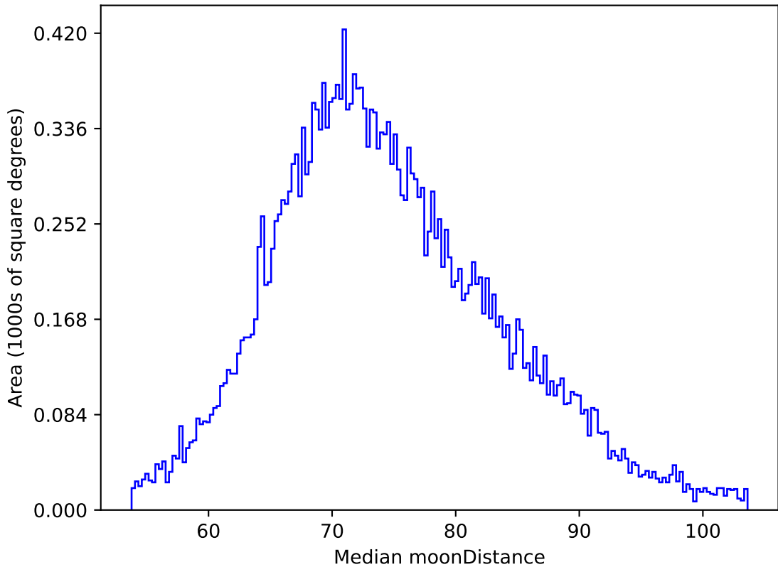
weather_cloudso0v3.4_10yrs All sky z band: Median moonDistance
