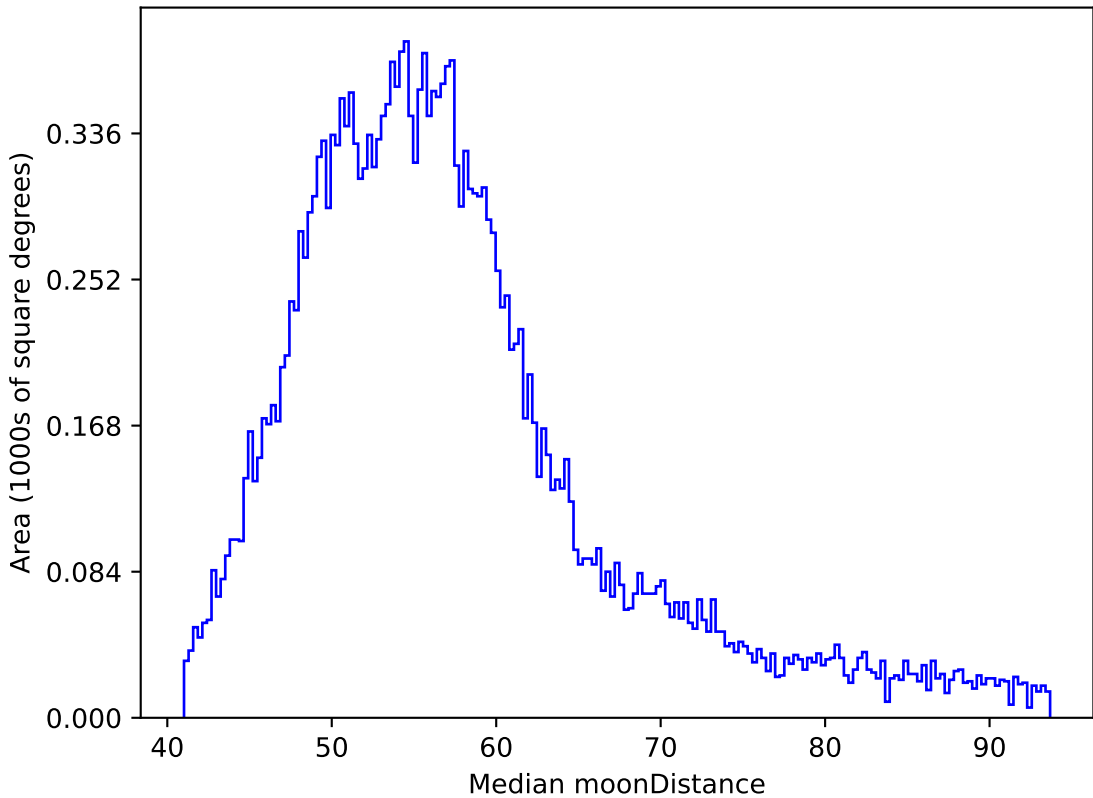
weather_cloudso0v3.4_10yrs All sky y band: Median moonDistance
