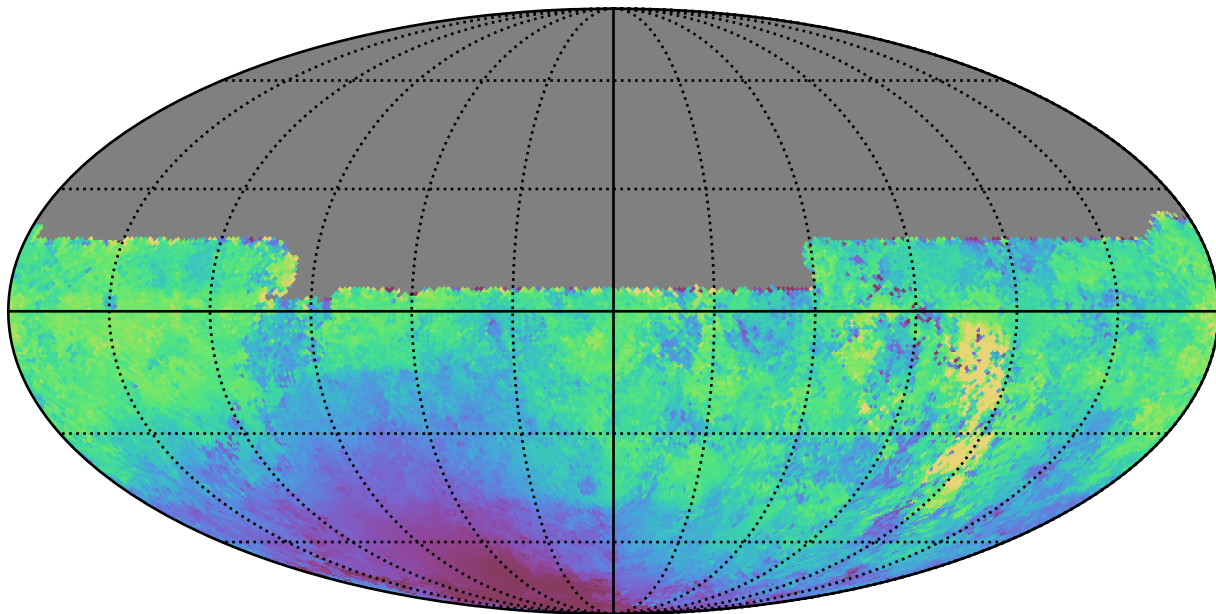
weather_cloudso0v3.4_10yrs All sky u band: Median moonDistance
