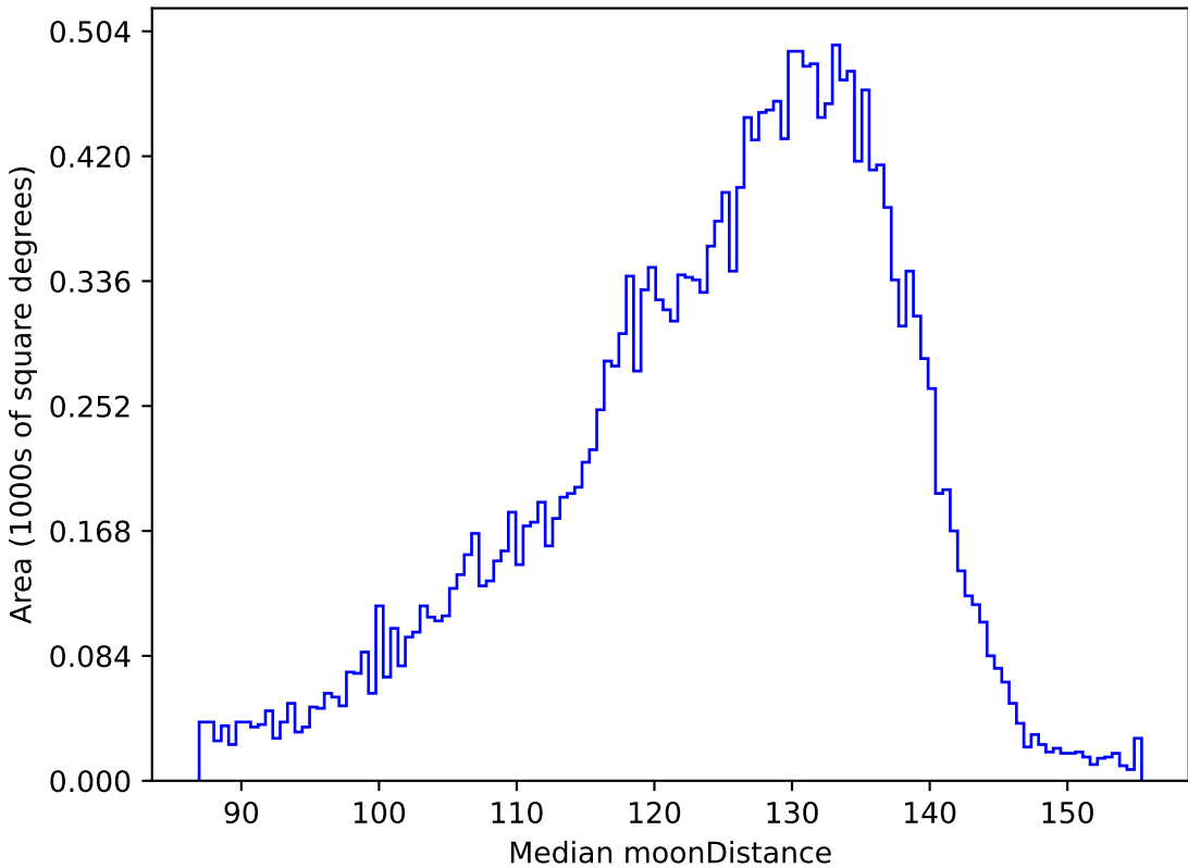
weather_cloudso0v3.4_10yrs All sky u band: Median moonDistance
