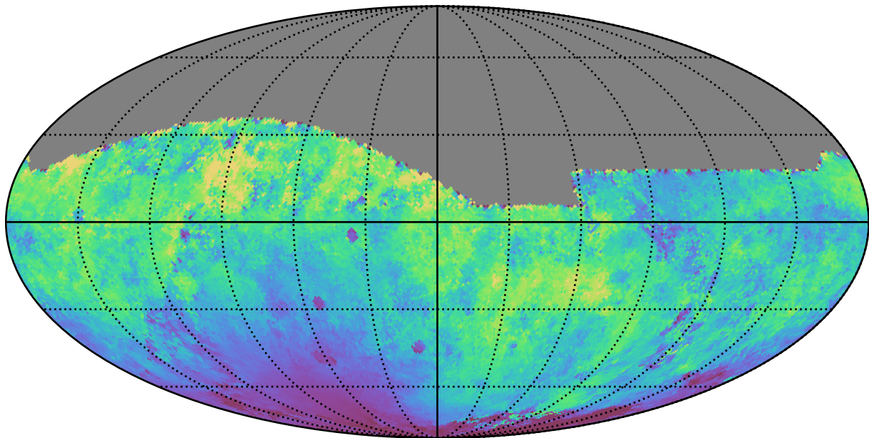
weather_cloudso0v3.4_10yrs All sky r band: Median moonDistance
