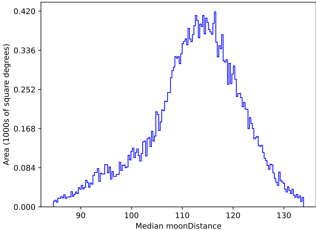
weather_cloudso0v3.4_10yrs All sky r band: Median moonDistance
