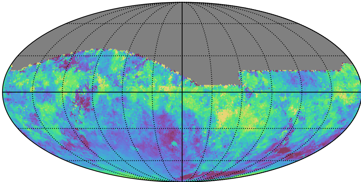
weather_cloudso0v3.4_10yrs All sky i band: Median moonDistance
