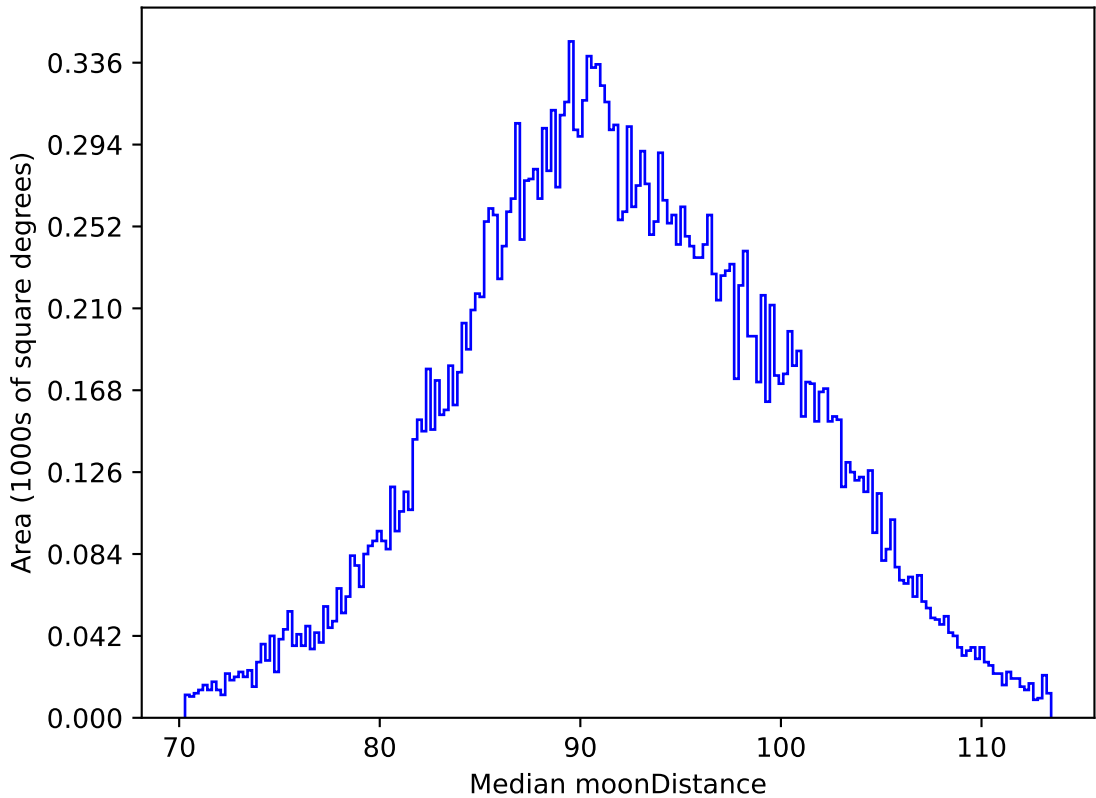
weather_cloudso0v3.4_10yrs All sky i band: Median moonDistance
