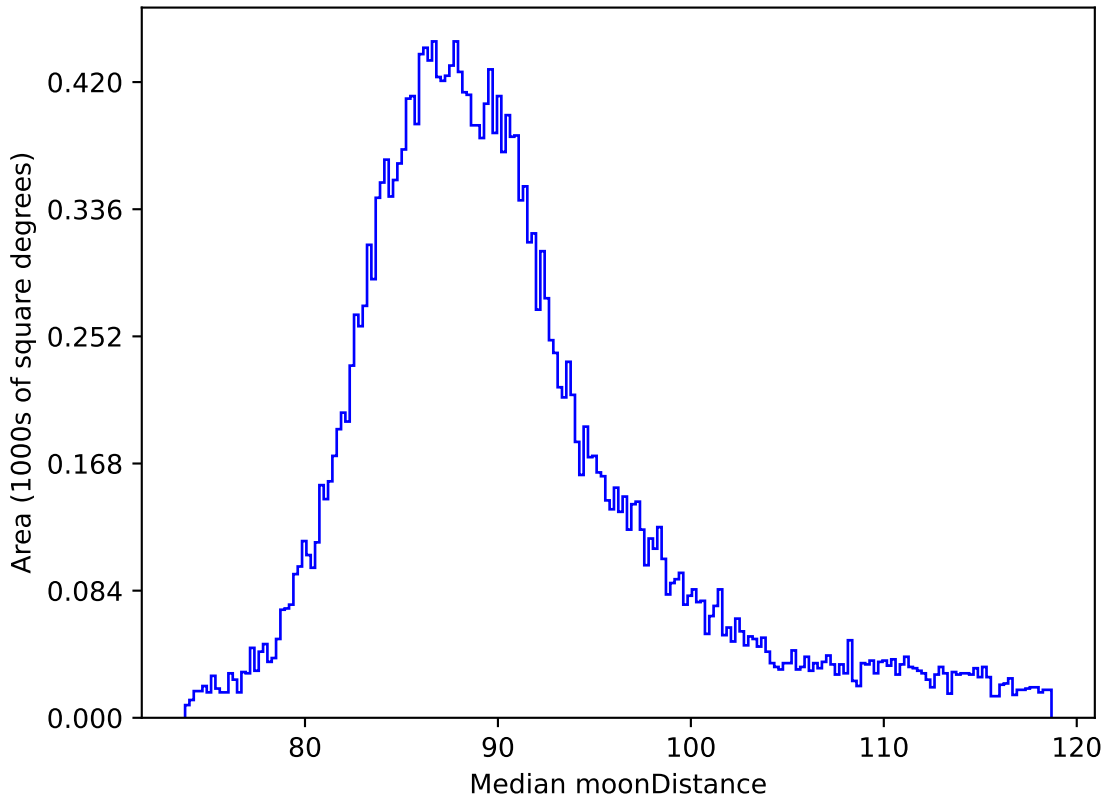
weather_cloudso0v3.4_10yrs All sky all bands: Median moonDistance
