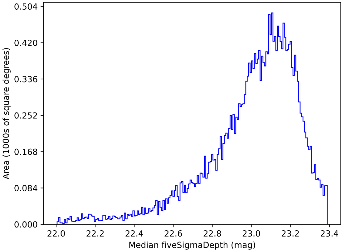
weather_cloudso0v3.4_10yrs Yr 1 z band: Median fiveSigmaDepth
