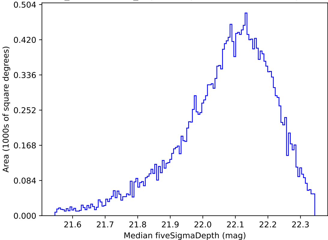
weather_cloudso0v3.4_10yrs Yr 1 y band: Median fiveSigmaDepth
