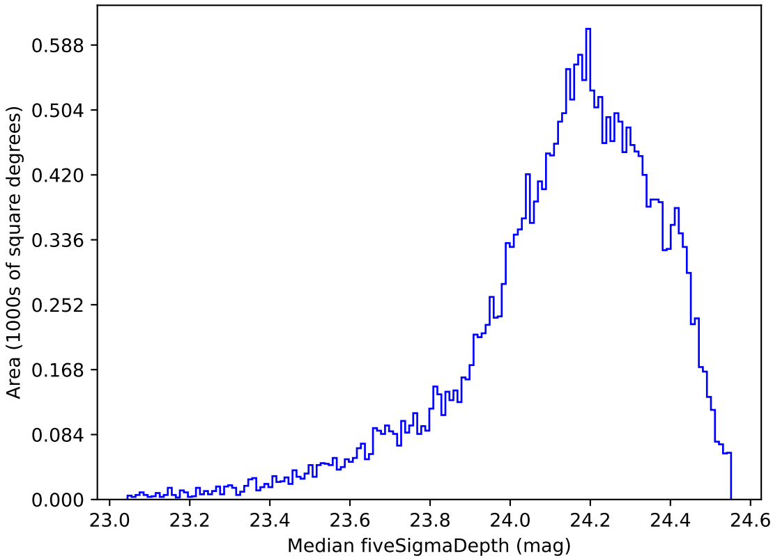
weather_cloudso0v3.4_10yrs Yr 1 r band: Median fiveSigmaDepth
