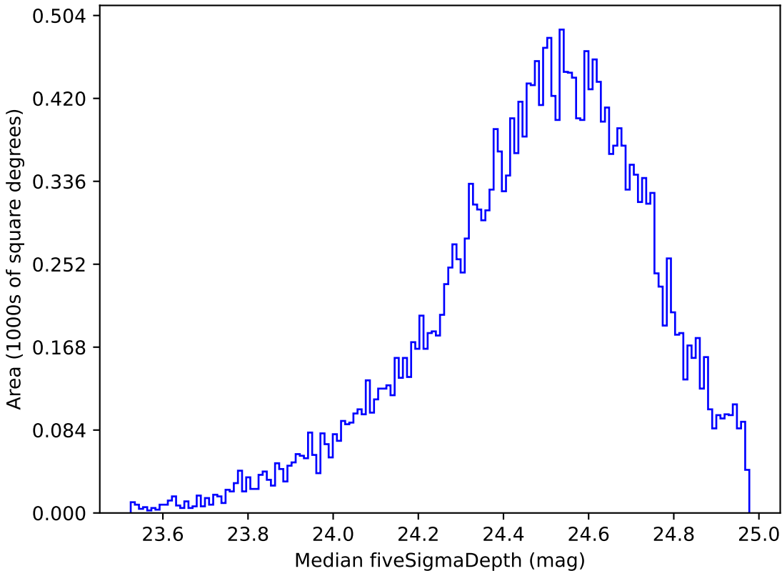
weather_cloudso0v3.4_10yrs Yr 1 g band: Median fiveSigmaDepth
