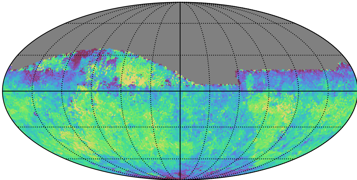
weather_cloudso0v3.4_10yrs Yr 1 all bands: Median fiveSigmaDepth
