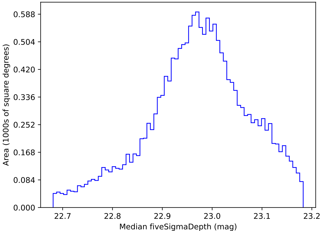
weather_cloudso0v3.4_10yrs WFD z band: Median fiveSigmaDepth
