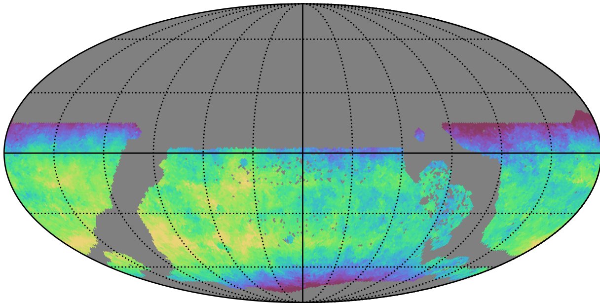
weather_cloudso0v3.4_10yrs WFD y band: Median fiveSigmaDepth
