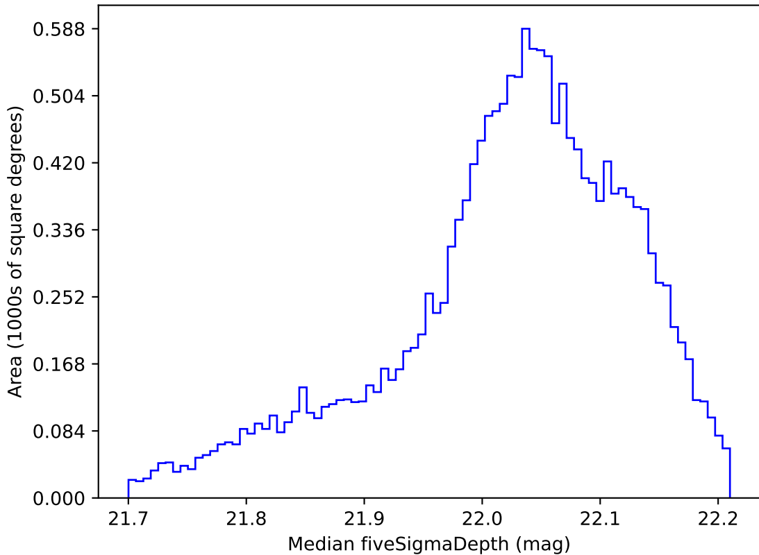
weather_cloudso0v3.4_10yrs WFD y band: Median fiveSigmaDepth
