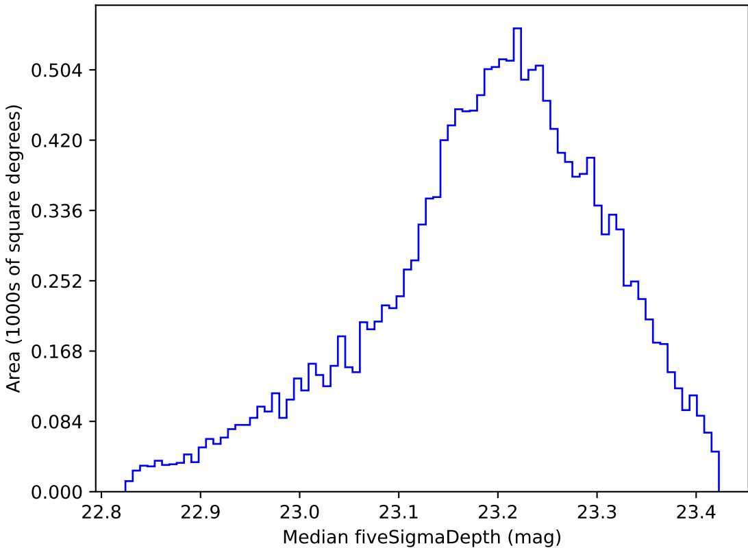
weather_cloudso0v3.4_10yrs WFD u band: Median fiveSigmaDepth
