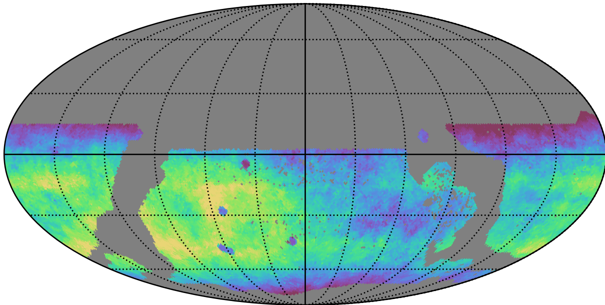
weather_cloudso0v3.4_10yrs WFD r band: Median fiveSigmaDepth
