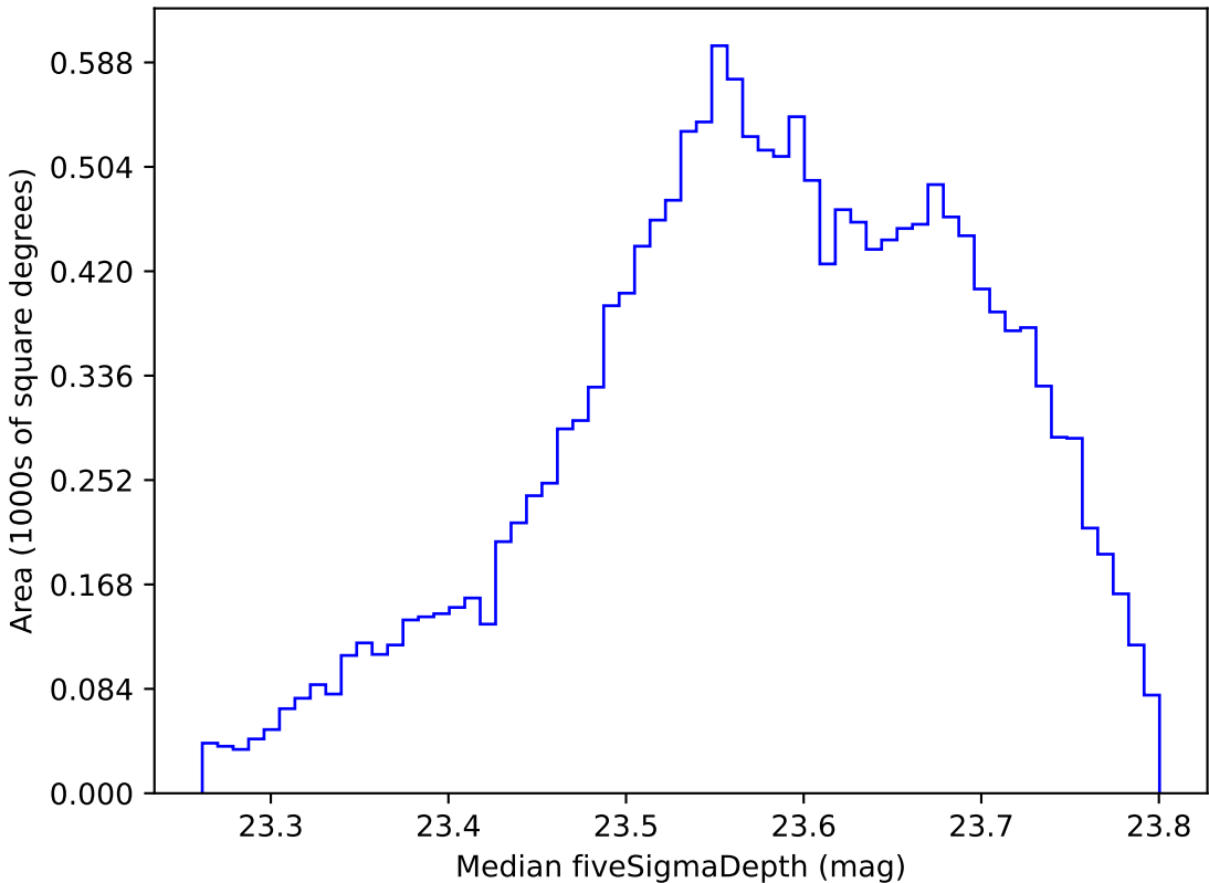
weather_cloudso0v3.4_10yrs WFD i band: Median fiveSigmaDepth
