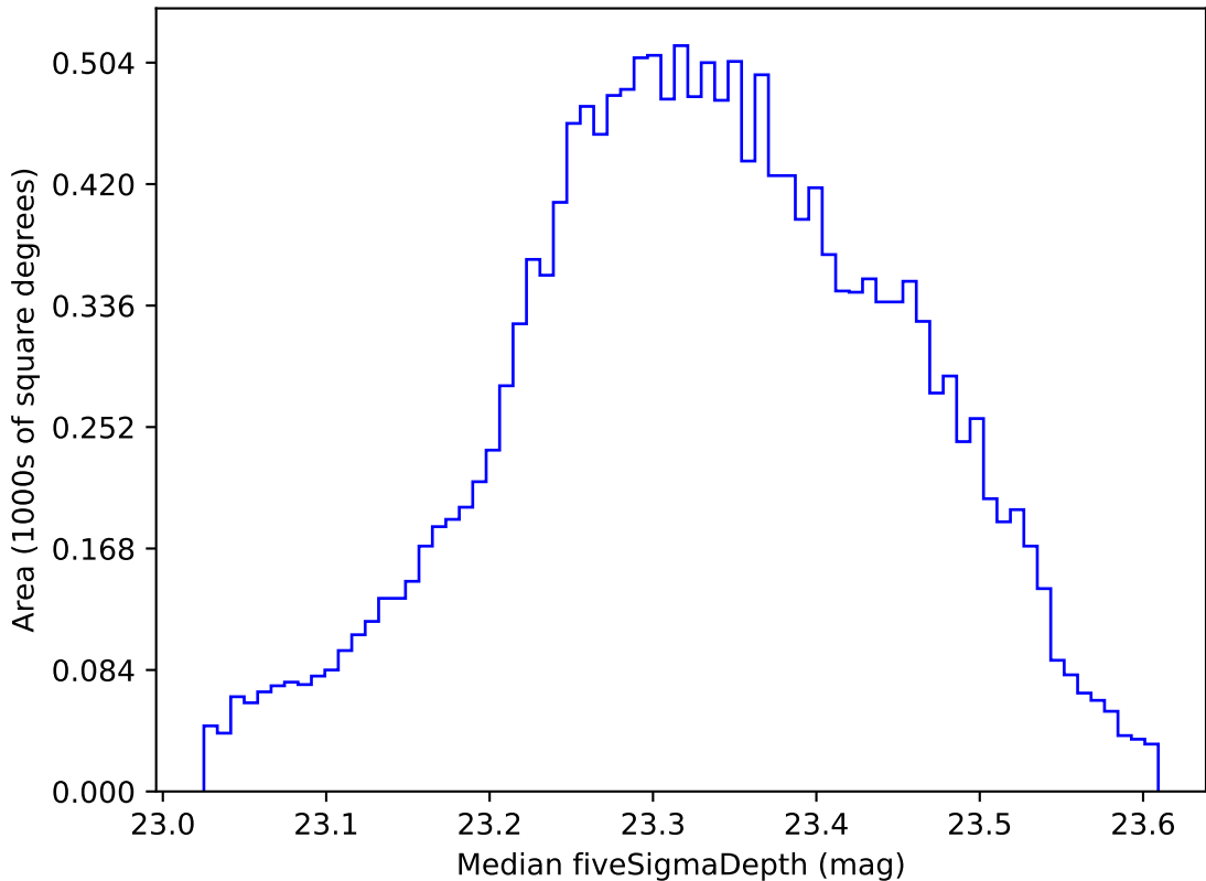
weather_cloudso0v3.4_10yrs WFD all bands: Median fiveSigmaDepth
