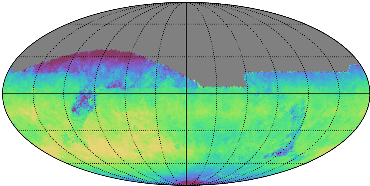
weather_cloudso0v3.4_10yrs All sky z band: Median fiveSigmaDepth
