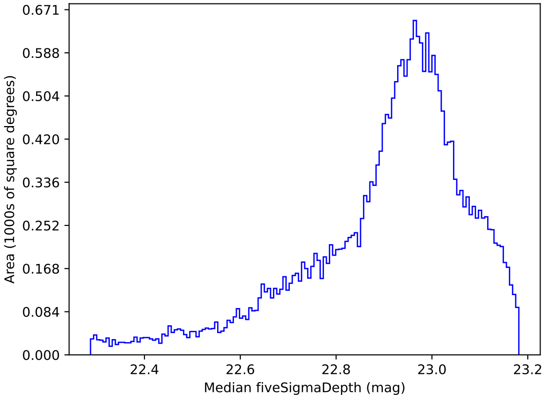
weather_cloudso0v3.4_10yrs All sky z band: Median fiveSigmaDepth
