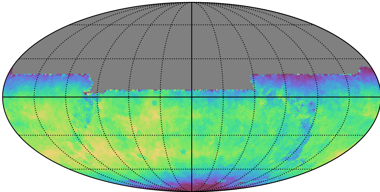
weather_cloudso0v3.4_10yrs All sky y band: Median fiveSigmaDepth
