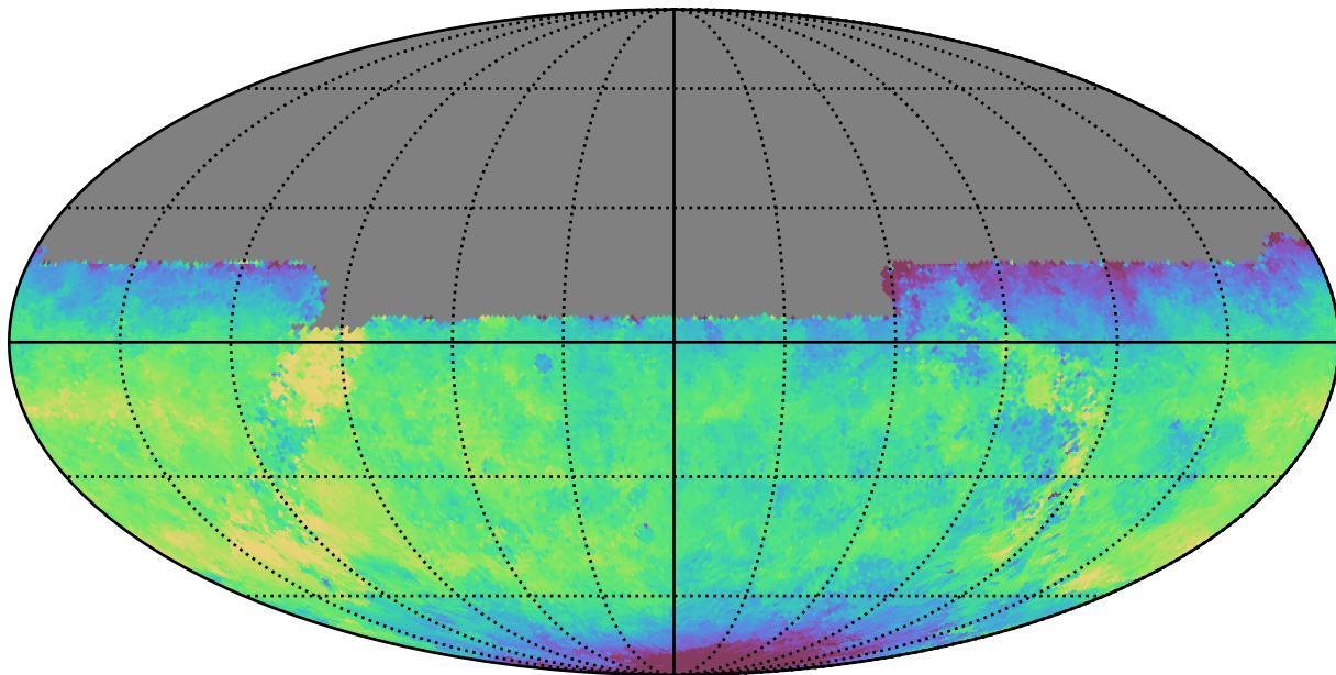
weather_cloudso0v3.4_10yrs All sky u band: Median fiveSigmaDepth
