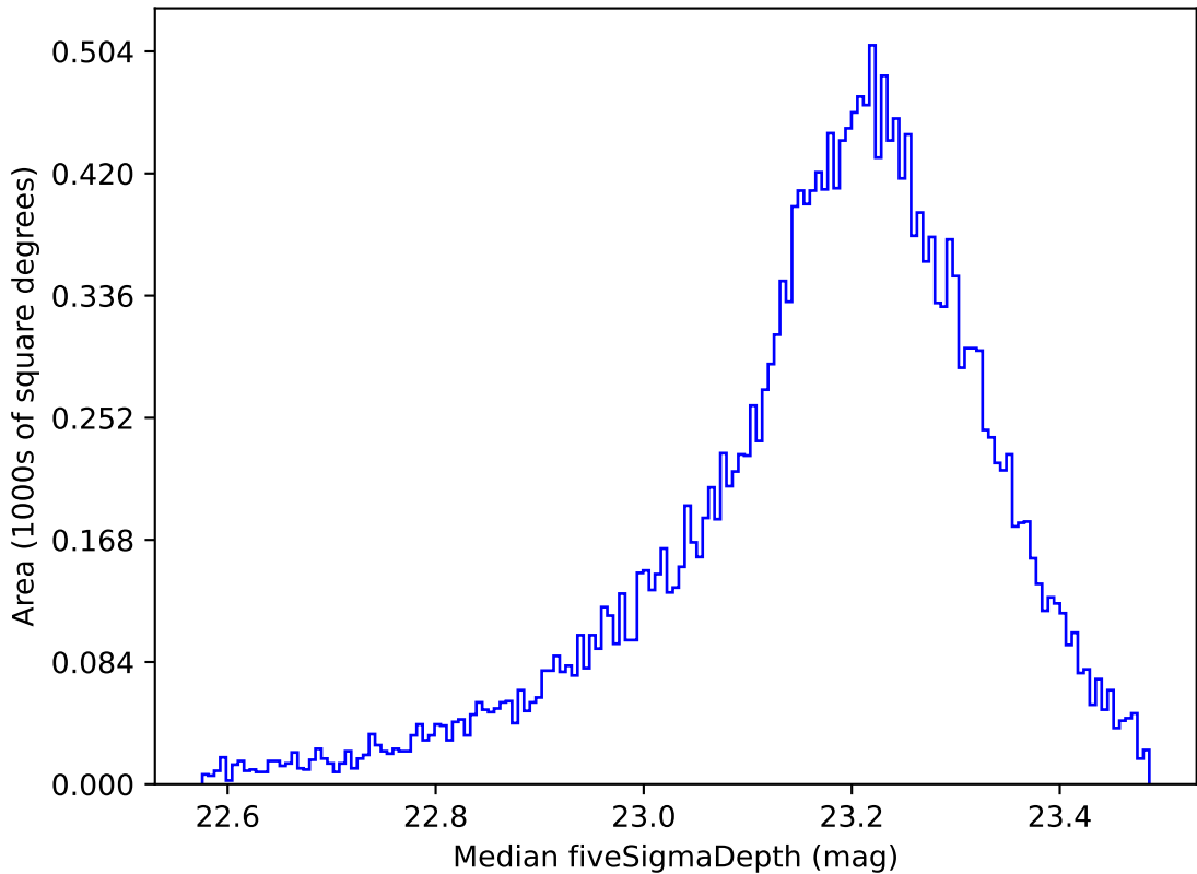
weather_cloudso0v3.4_10yrs All sky u band: Median fiveSigmaDepth
