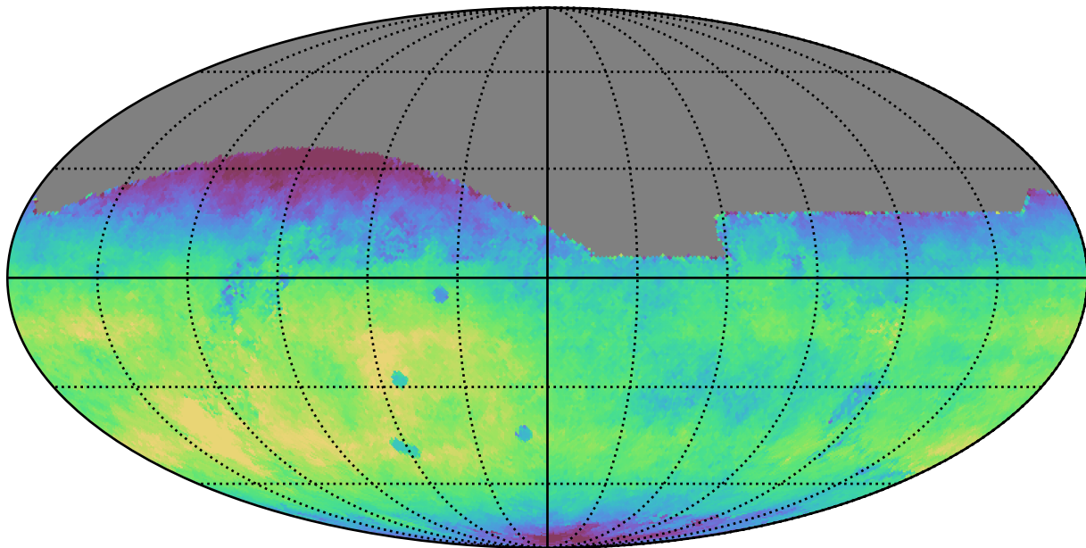
weather_cloudso0v3.4_10yrs All sky r band: Median fiveSigmaDepth
