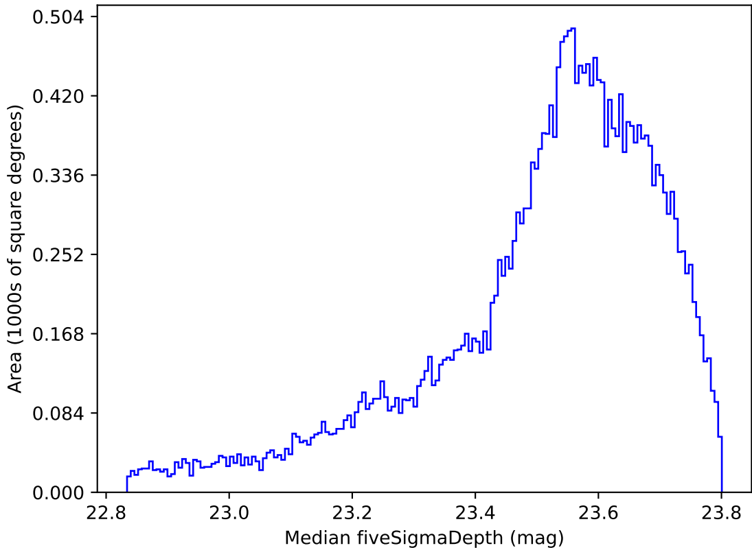
weather_cloudso0v3.4_10yrs All sky i band: Median fiveSigmaDepth
